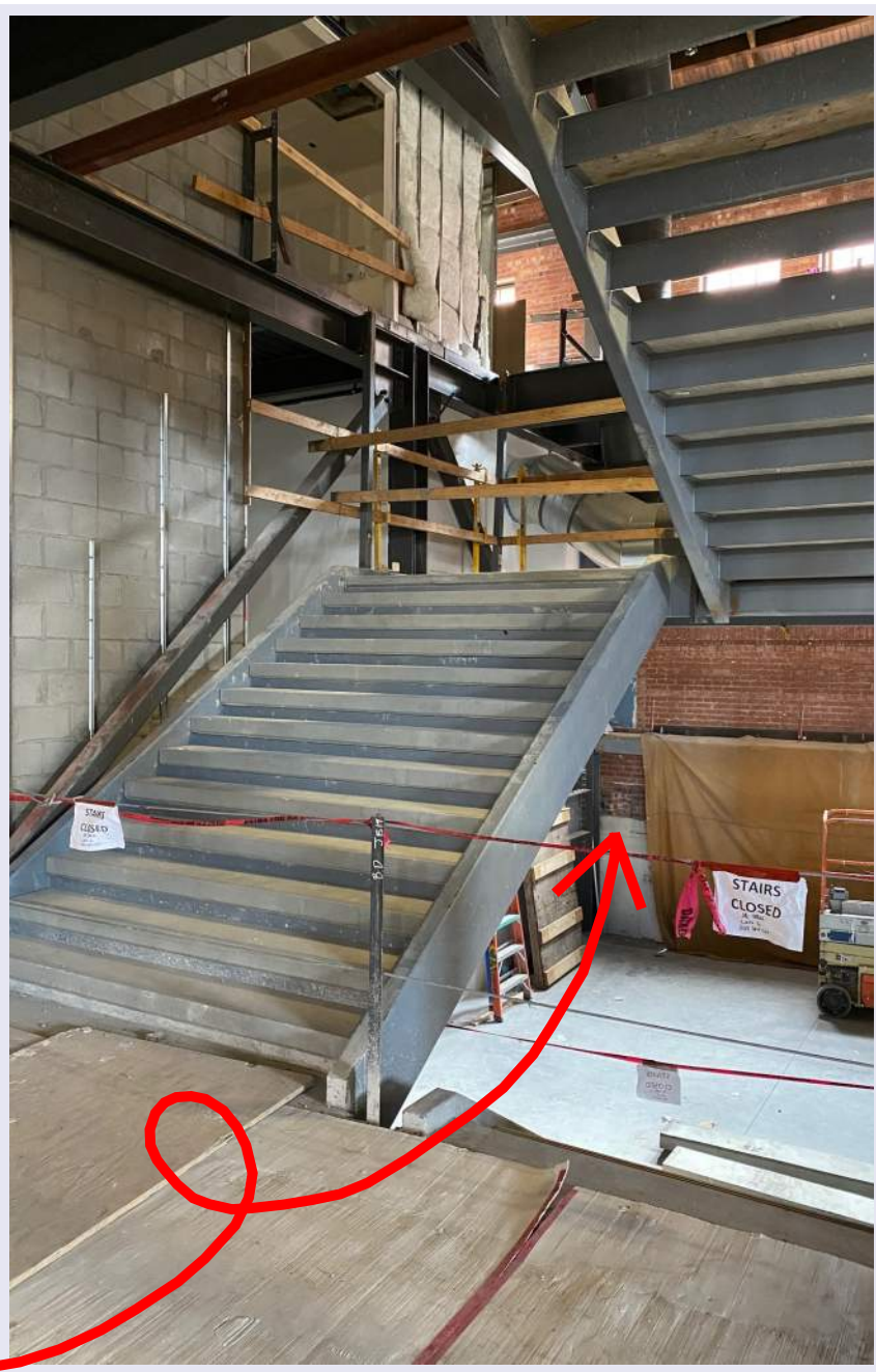
On the left, the exterior receives concrete patch work around two new louvers for the mechanical system. On the right, the precast stair treads are continuing to be installed!
