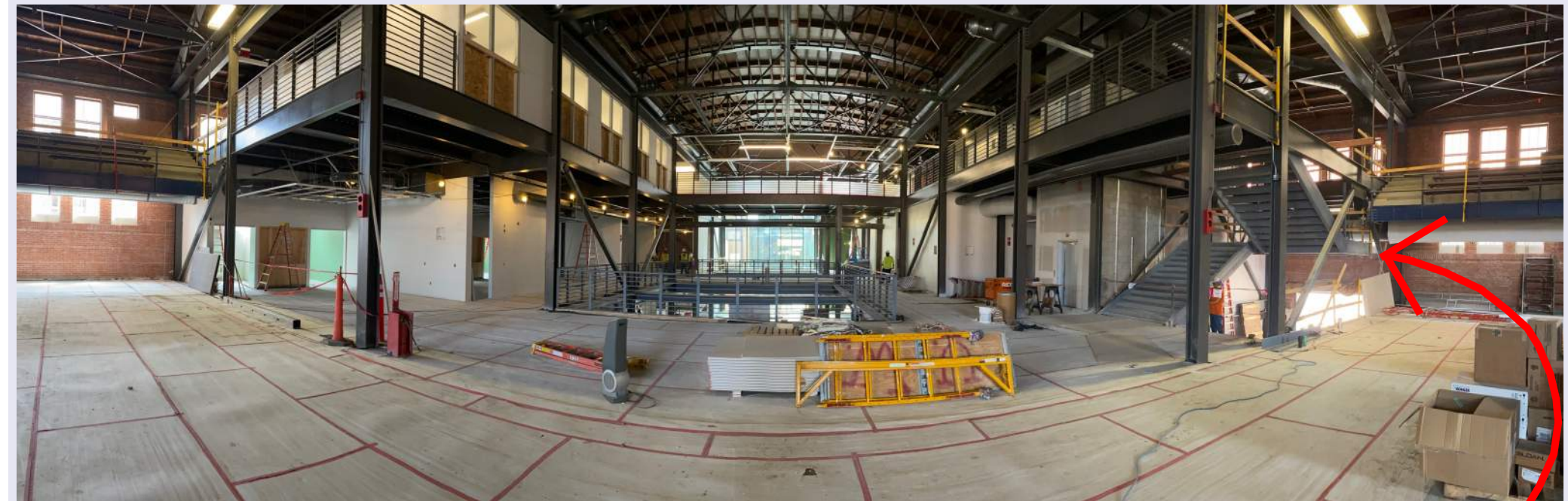
Inside the main entrance standing on the historic gym floor, looking south. Lighting fixtures are going in on level 3, acoustical ceilings are finishing up on level 2, and the catering kitchen is being framed on level 1.
